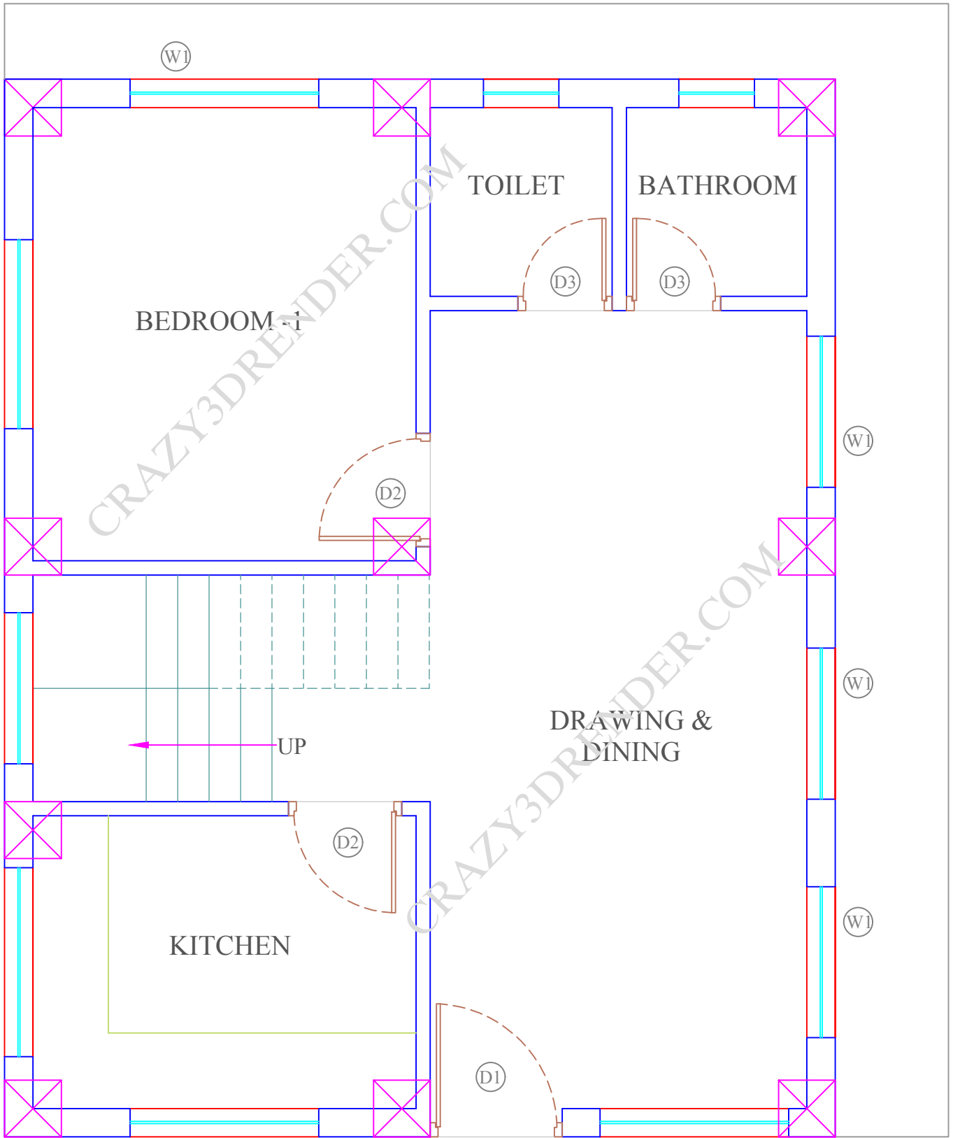
COLUMN PLAN
