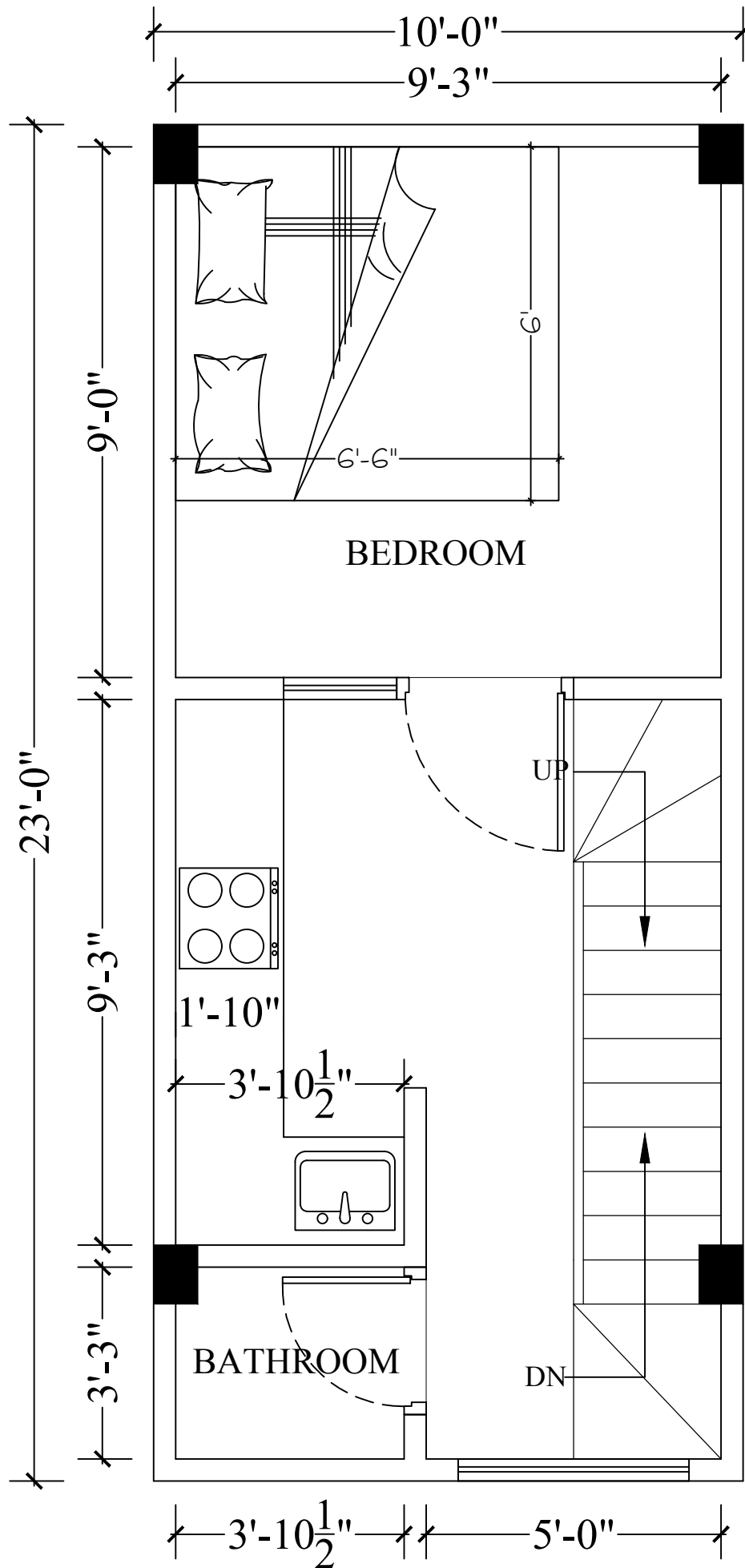
FIRST FLOOR
